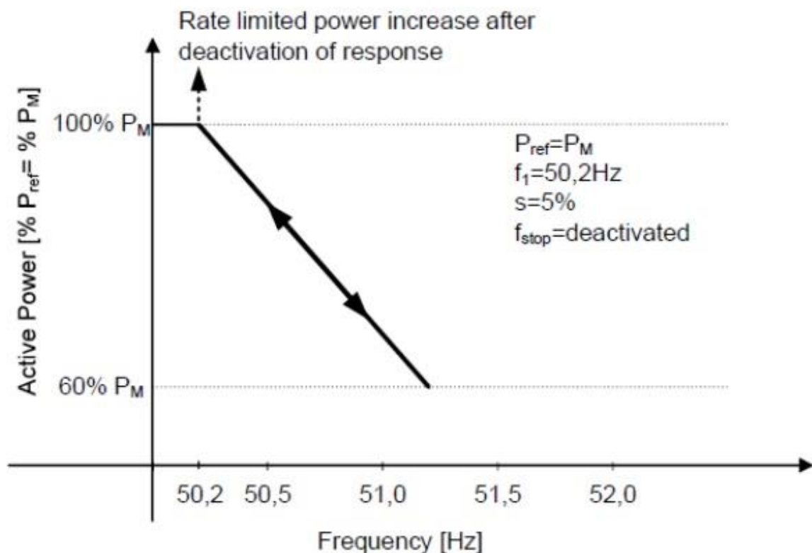
Figure 3: Autonomous P(f) characteristics - example
